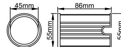
Back Box
