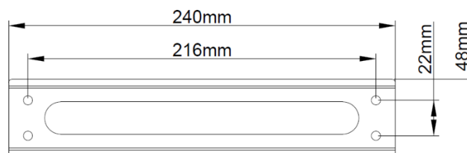
Back plate & Fixing Dimensions.
