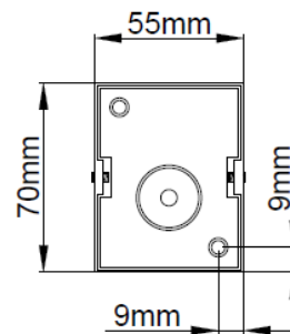
Back plate Details.
